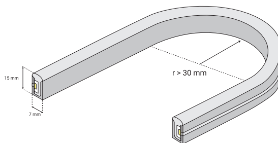
Fig. 2. Drawing of the minimum bend radius.
