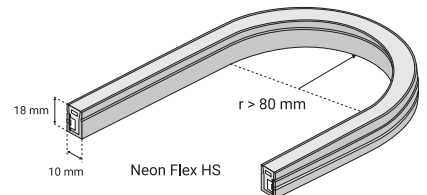
Fig.2. Drawing of the minimum bend radius.
