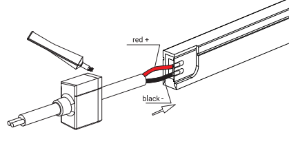
Fill the forward end cap with silicon glue, and then seal to the strip body.
