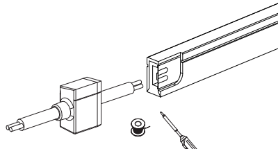
Solder the cable to the bottom solder pad.
