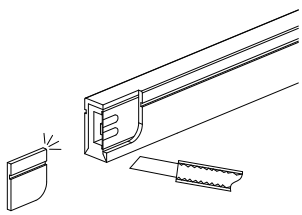
Peel off some part of silicone in 3mm[0.12in.], to bare the bottom solder pad.
